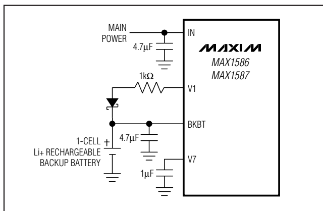
Figure 9. A 1-cell rechargeable Li + battery provides more backup power when a primary cell is insufficient. The cell is charged to 3.3V when V1 is active. Alternately, the battery can be charged from IN if the voltages are appropriate for the cell type.
